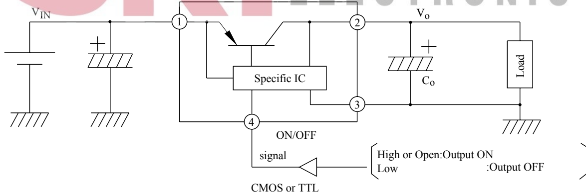
Fig. 2 Application Circuit for Standard
